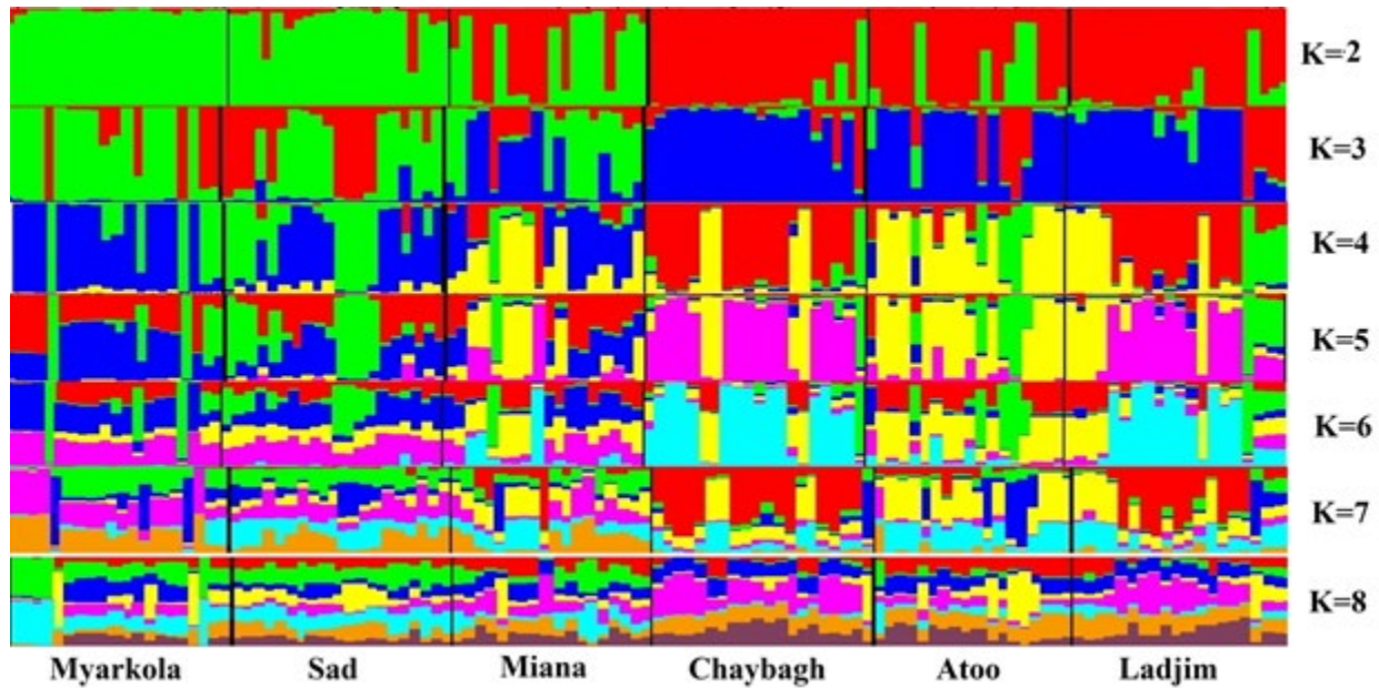
Fig. S1. Bayesian clustering results obtained with Structure, for K = 2 to K = 8 , for Pterocarya fraxinifolia in the Hyrcanian Forest.
