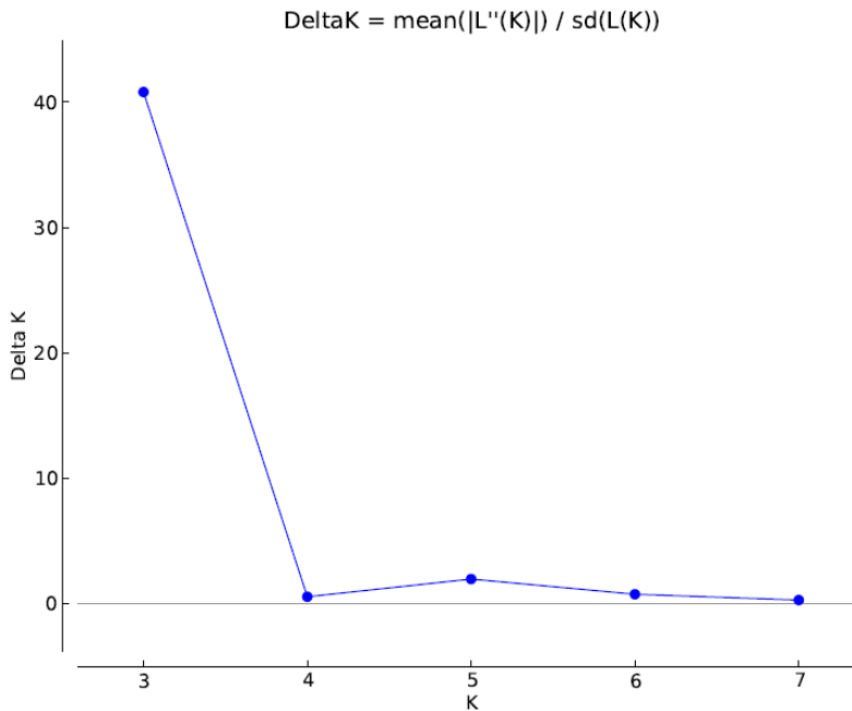
Fig. S2. Estimated number of populations ( K ) for Pterocarya fraxinifolia from Structure analysis.
