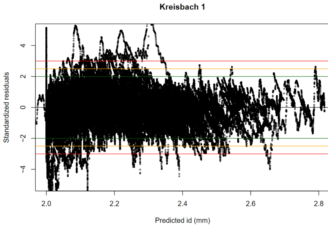
Figure S7-2. Standardized residuals for model Kreisbach 1
