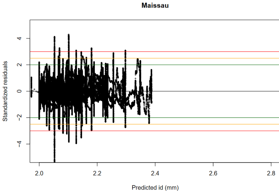
Figure S7-1. Standardized residuals for model Maissau
