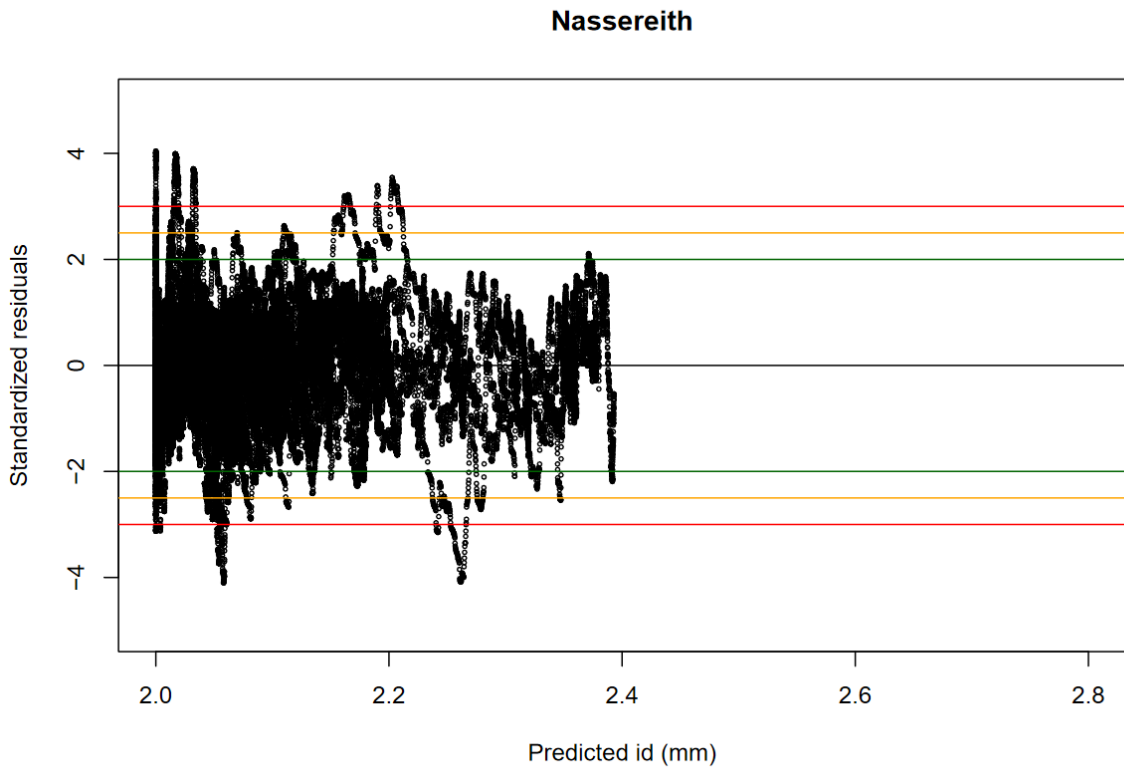
Figure S7-4. Standardized residuals for model Nassereith
