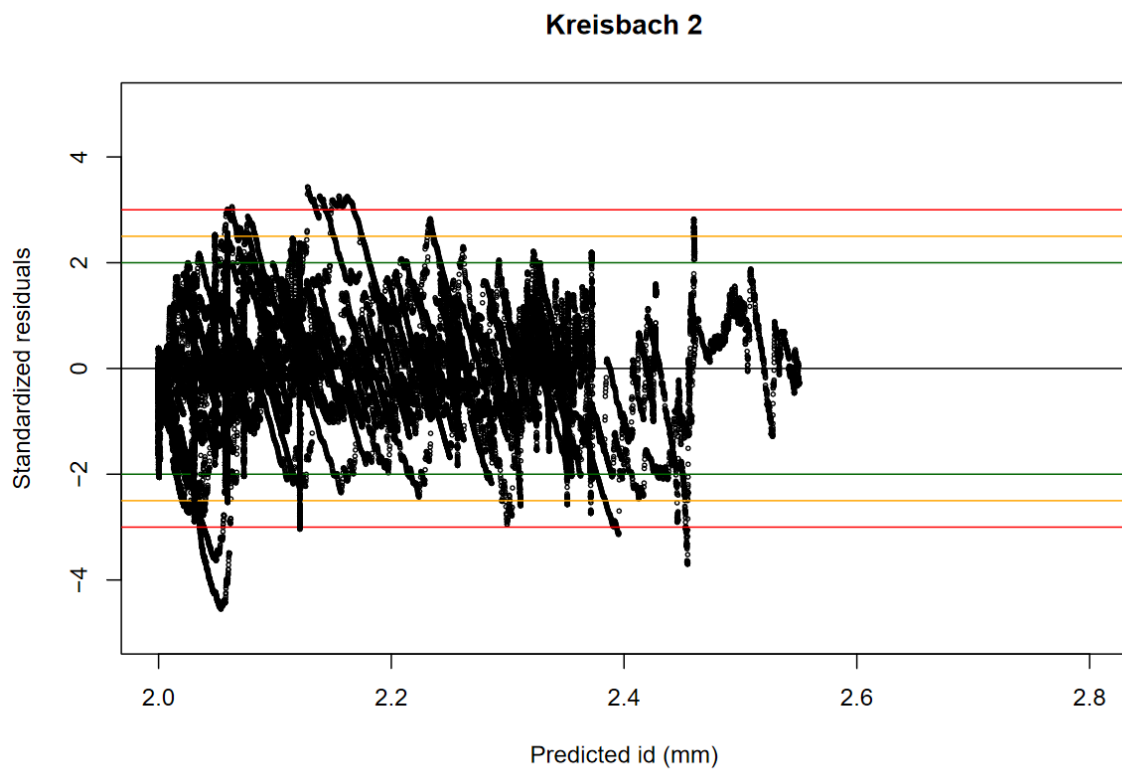
Figure S7-3. Standardized residuals for model Kreisbach 2
