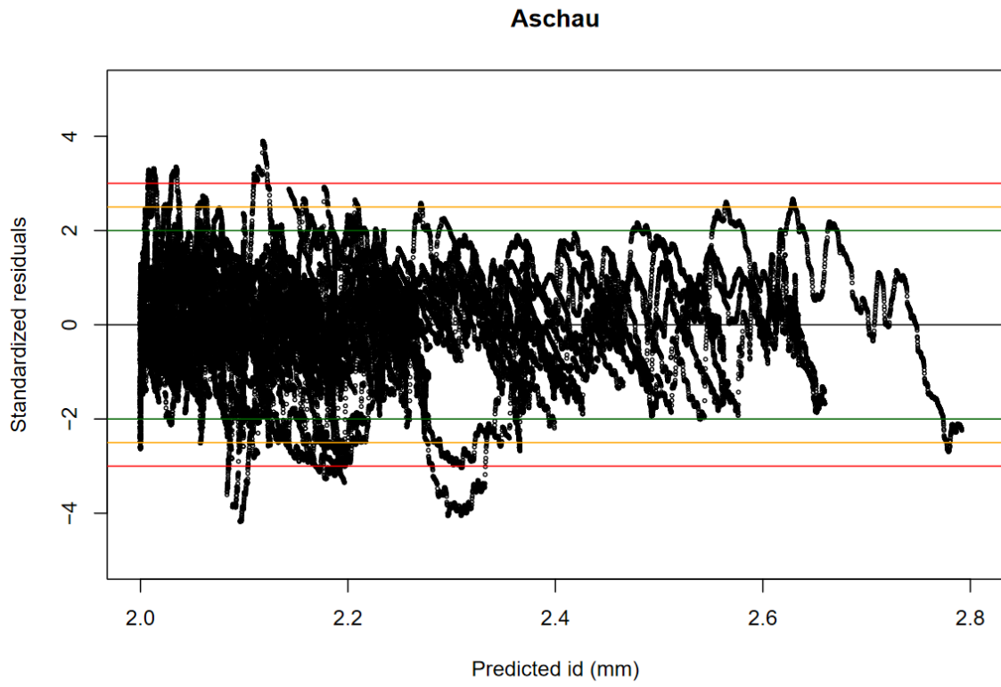
Figure S7-6. Standardized residuals for model Aschau
