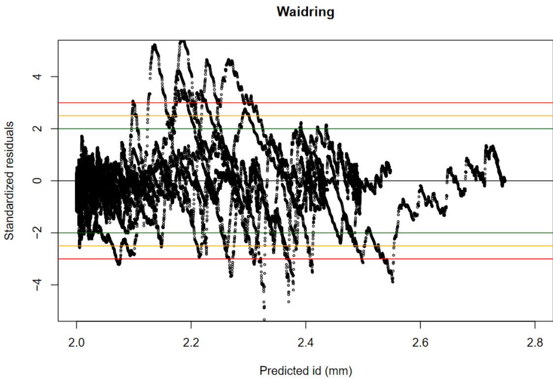
Figure S7-5. Standardized residuals for model Waidring
