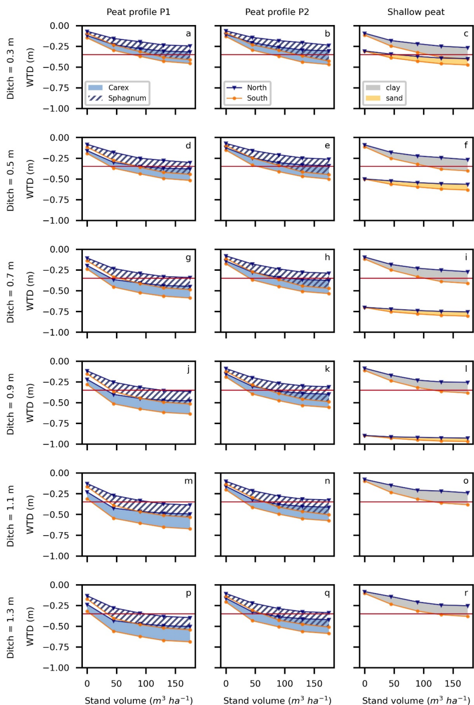
Figure S3. Median of July-August WTDs (m) for different peat profiles (P1, P2 and shallow peat) with various ditch depths and stand volumes with ditch spacing of 50 m. The shaded or hatched area represents the range in simulated climatic conditions; the lower limit (orange dots) represents the southernmost and upper limit (blue triangles) represents the northernmost climate. In subfigures o and r, the WTD for sand subsoil profile falls below -1 m and is thus not shown. The red lines mark the -0.35 m WTD.
