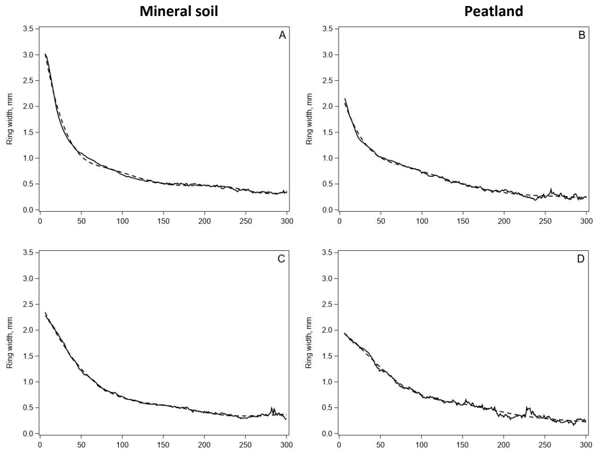
Fig. S2. The regional curve standardisation (RCS) curve was calculated by averaging the tree-ring widths according to their age counted from the pith outwards (continuous line) and the mean of all the series was modelled by a stiff spline (dashed line) for Scots pine (upper row) and Norway spruce (lower row) in North Finland.
